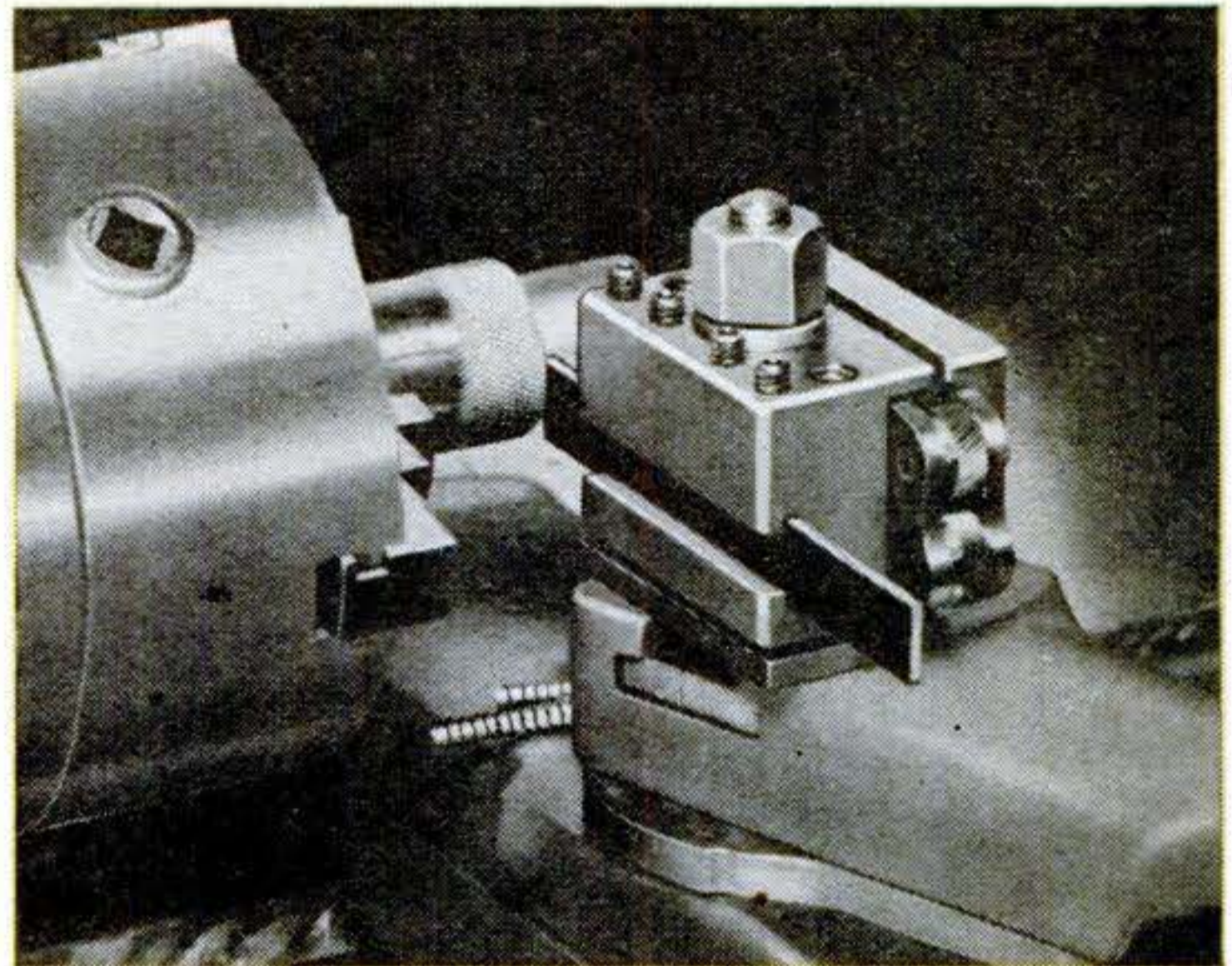
Universal Tool Block
